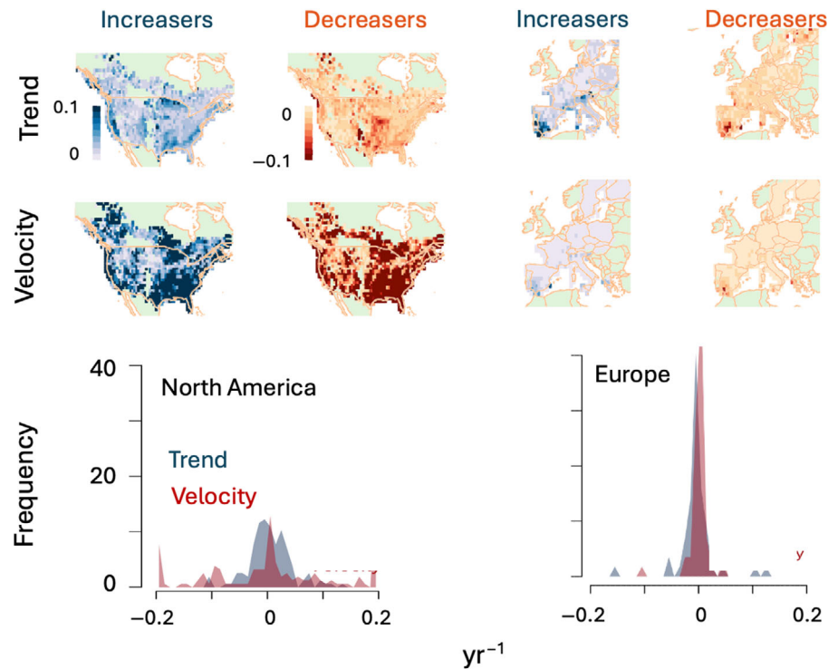
Fig. 4 Trends and response velocities, shown separately as averages for species that had increasing fecundity (blue maps) and decreasing fecundity (red maps). Trends and velocities are aggregated over species at the bottom. The similarities between trend and velocity in these aggregate maps disappear at the species level due to high noise in time-series data used to estimate trends (Supporting Information Figs S4, S5).
