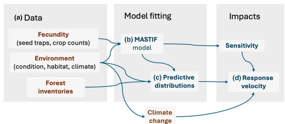
Fig. 2 Analysis consists of data collections (a), model fitting (b), and generation of predictive distributions for forest inventory plots (c), and evaluation of response velocities (d).
